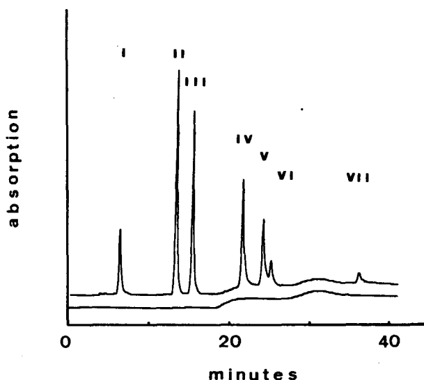
FIGURE 1 Co-chromatography of s -triazines in diluted waste-water with authentic s -triazines. The experiment was done at room temperature at a flow-rate of 0.8 ml/min. A stepped gradient was used. The first solvent (100 mM potassium phosphate buffer, pH 6.7) was delivered for 4 minutes, when a linear gradient to 70% of the second solvent (70% methanol, 30% 10 mM potassium phosphate buffer, pH 6.7) over 10 minutes was applied. After a further 10 minutes, the gradient was resumed to give 100% of the second solvent over 5 minutes. The lower line in the figure is the blank, obtained without injection of sample.
